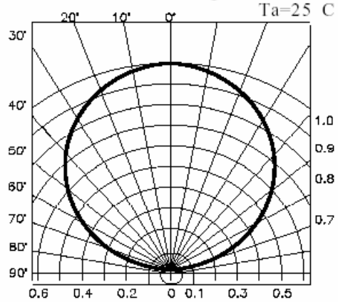
Radiation Diagram
